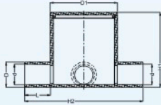
DEEP J/BOX with 3 way entries
