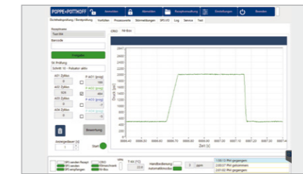
Figure 2: Trapezoidal test curve
