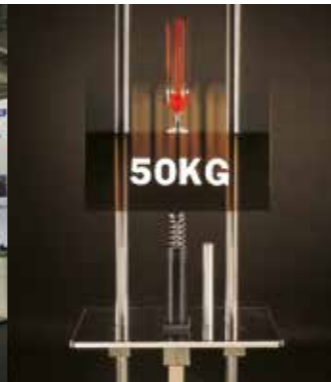
ACE drop tester – a wine glass dropping free fall 1.3 m. Decelerated by a shock absorber not a drop of wine is spilled.
