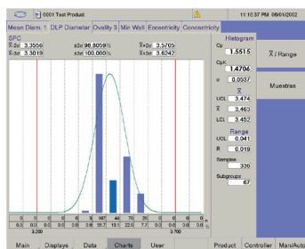
Histogram
