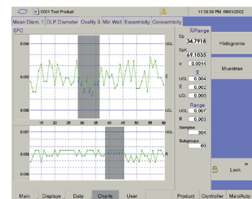
SPC charts
